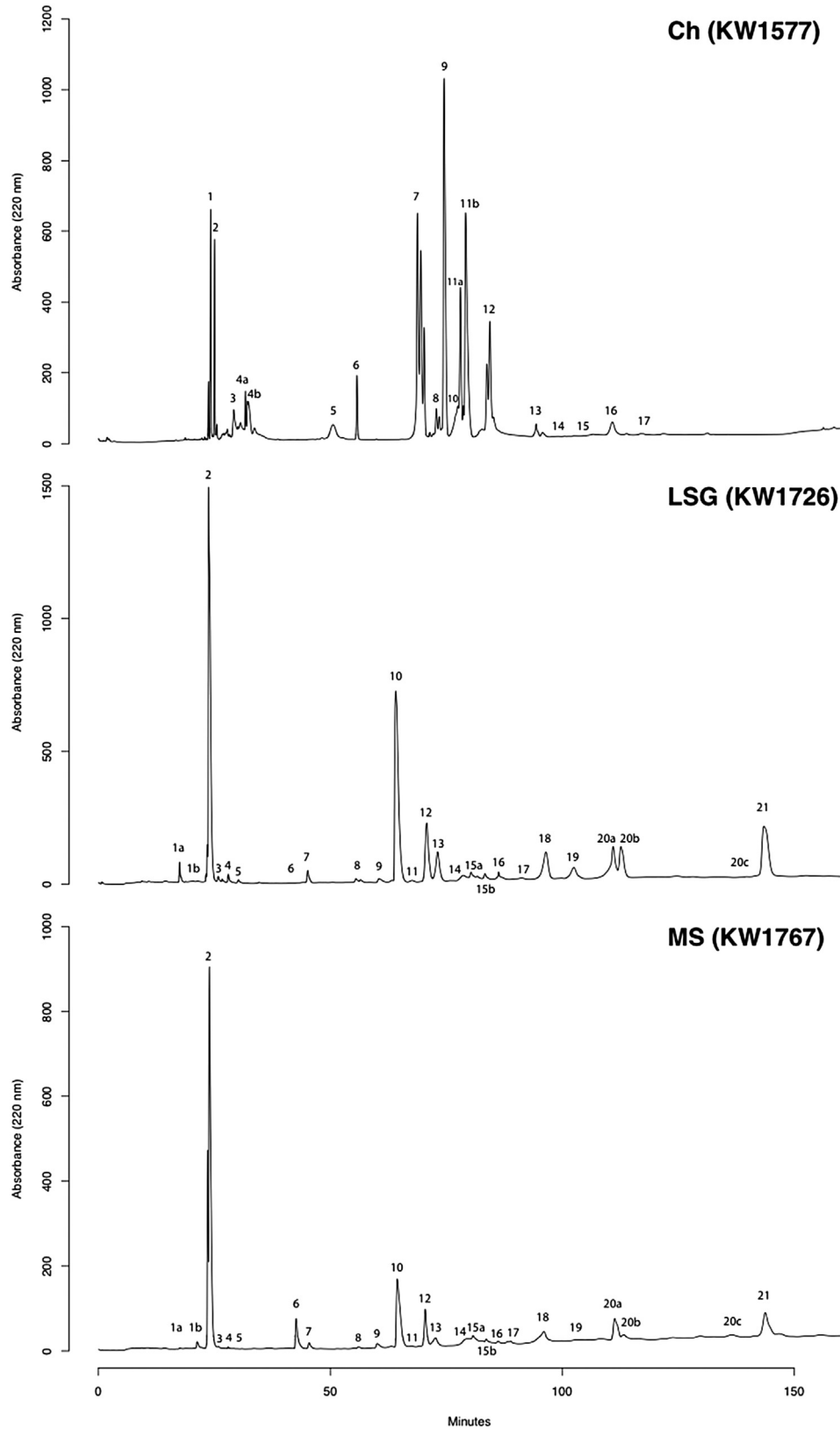
Fig. 3. Representative chromatograms of individuals from each cohort. KW numbers in parentheses refer to the sample identifications in Table 1. Time scale is the same for all three cohorts.
