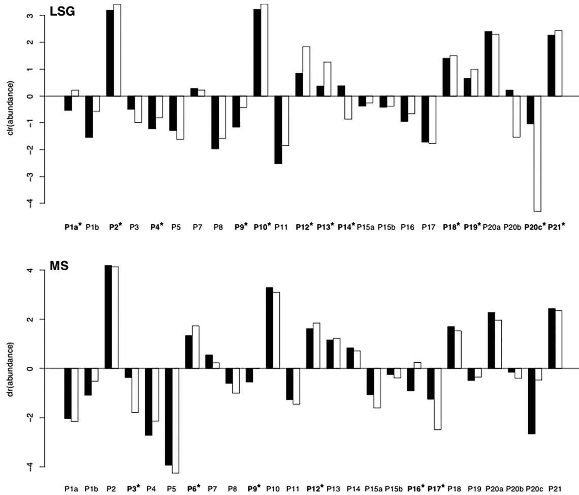
Fig. 1. Mean centered log ratio expression levels from two litters of Crotalus adamanteus : Little St. George (LSG; n = 6 ) and Mississippi (MS; n = 8 ). These values represent the clr transformation of the average venom. Peaks that displayed statistically significant changes are in bold and marked with an asterisk (see also Tables 1 and 2). Black bars = before postnatal shed, white bars = after postnatal shed. Note: Peak six was absent in LSG and so was not included.
