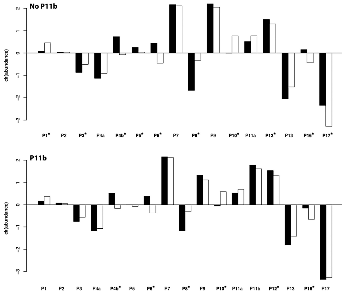
Fig. 2. Mean centered log ratio expression levels from a litter of Crotalus horridus divided into two groups: individuals without peak 11b ( n = 9 ) and those with peak 11b ( n = 8 ). These values represent the clr transformation of the average venom. Peaks that displayed statistically significant changes are in bold and marked with an asterisk (see also Tables 1 and 2). Black bars = before postnatal shed, white bars = after postnatal shed.
